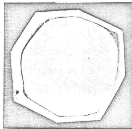
Fig. 1. Silver iodide in diamond anvil high-pressure cell at an applied pressure of 4 kb ( \times 100 ).
